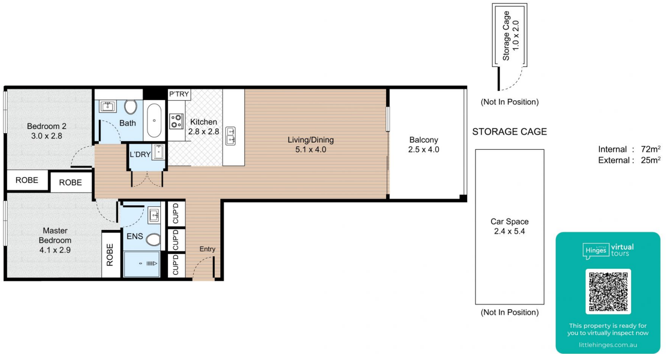
FLOOR PLAN
