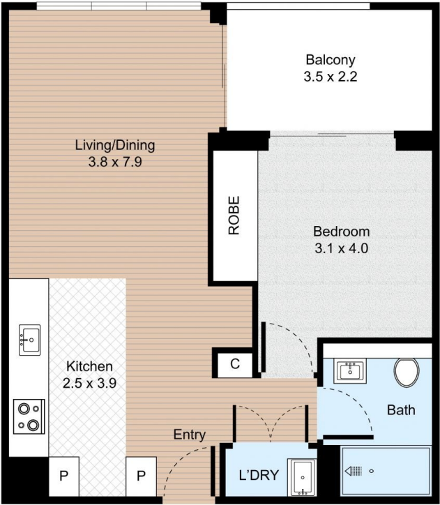
FLOOR PLAN
